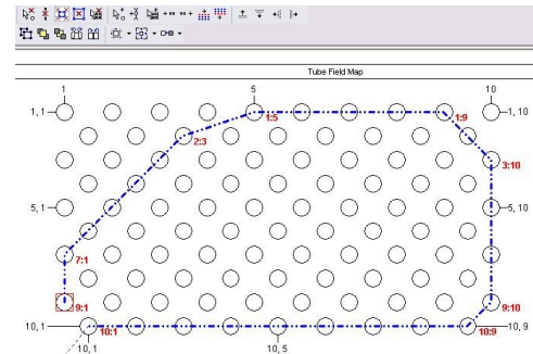
TubePro 3D User Interface
